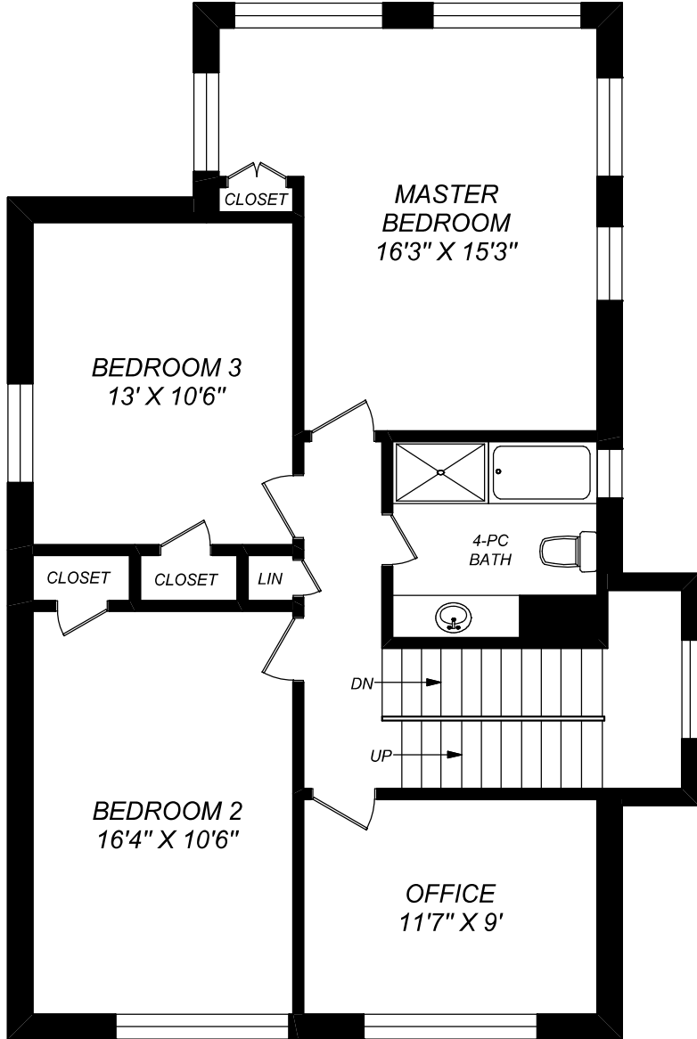
SECOND FLOOR 1005 SQUARE FEET
